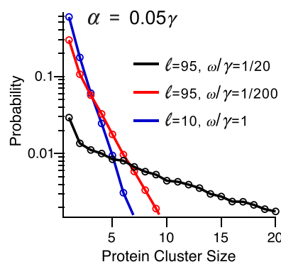
Fig. 7. The effect of having different levels of secretory machinery for \alpha = 0.05\gamma , L = 100 , and PSR sizes of \ell = 10 and \ell = 95 . It is seen that the distribution of protein cluster size can vary greatly depending on the availability of secretory machinery.
